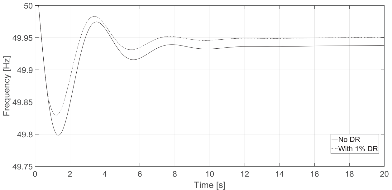
Figure 12. Impact of dynamic demand response on system frequency
