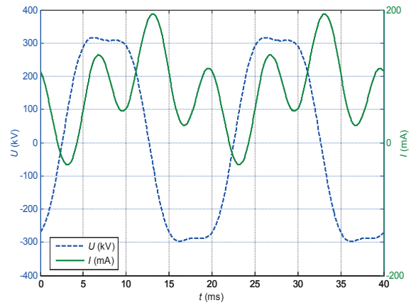
Figure 12. U - I waveforms for I_{DC}=80 mA
