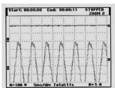
Slika 11 — Kratki spoj generatora: uzbudni napon uzbudnika i struja armature PMG-a Figure 11 — Generator short circuit: field exciter voltage and PMG armature current
