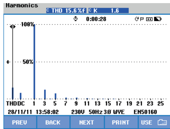
B. Harmonic Spectrum of Current Harmonics in B Phase.
