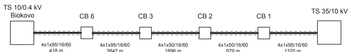
Figure 3. Schematic diagram of the 10 kV cable line
