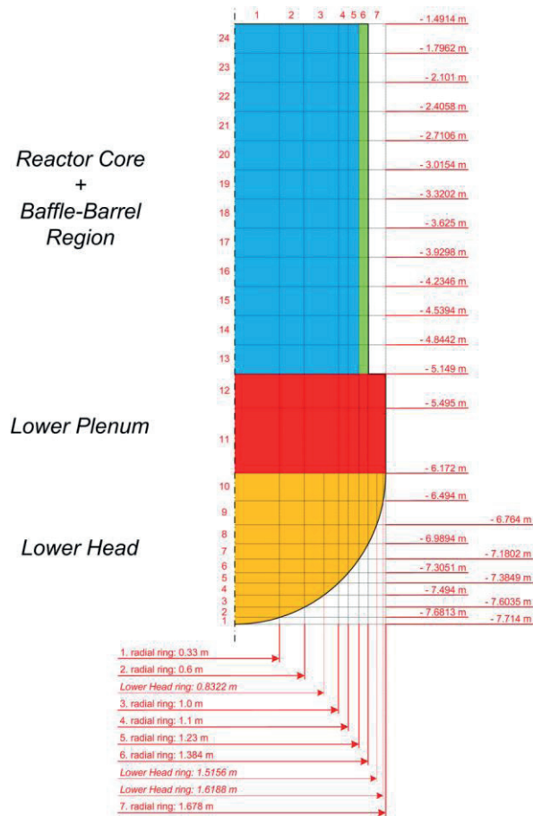
Figure 2: Axial representation of the reactor core and the lower plenum used in the COR package
